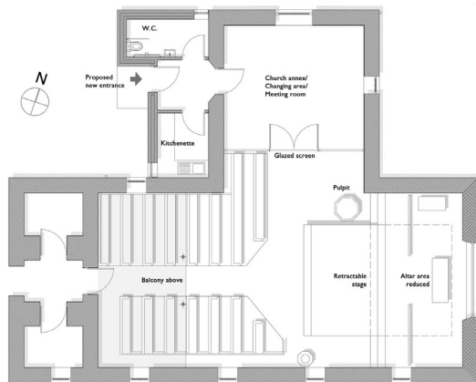
Floor plan showing the proposed extension
